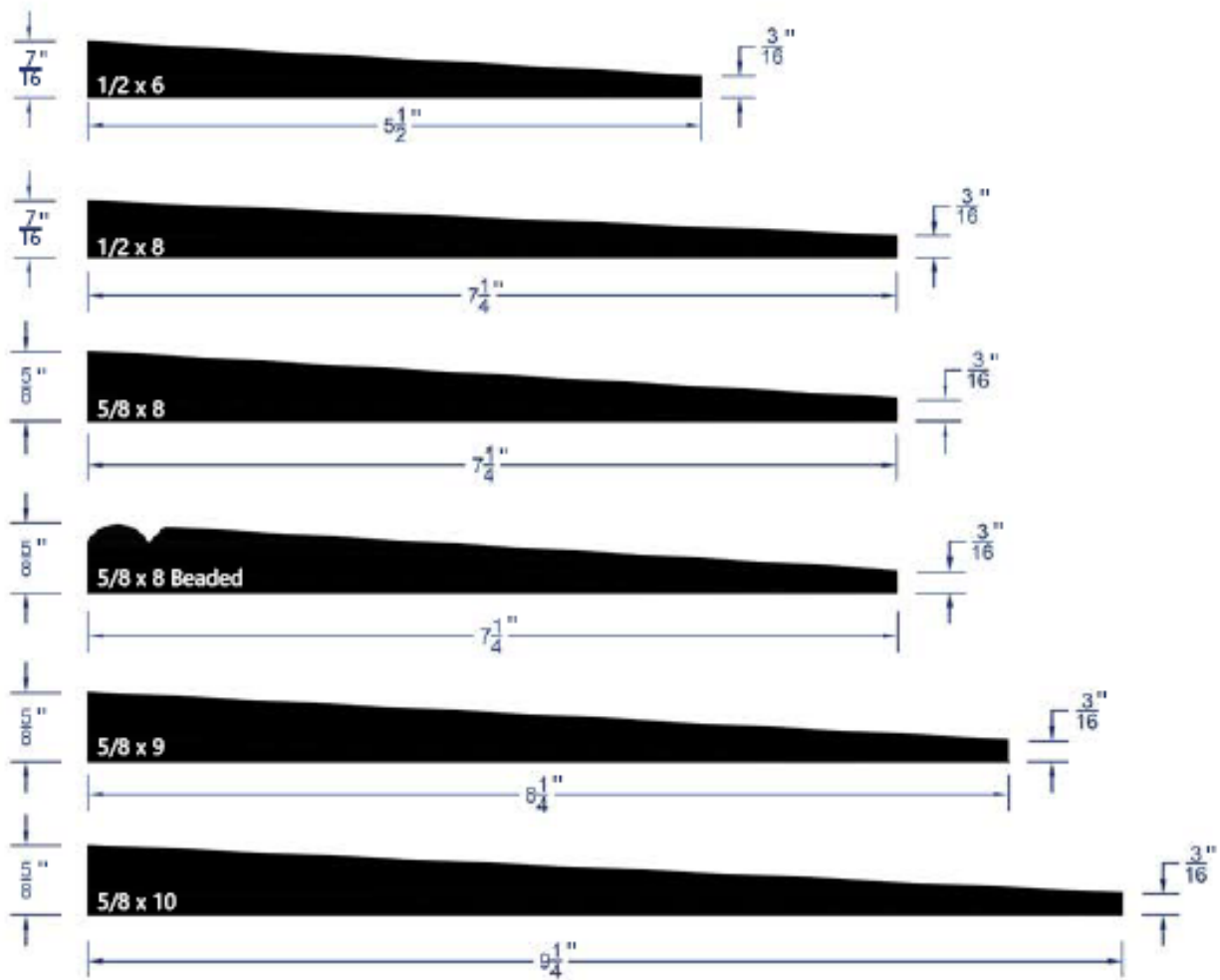
FIGURE 1 – DURATION BEVELED SIDING
