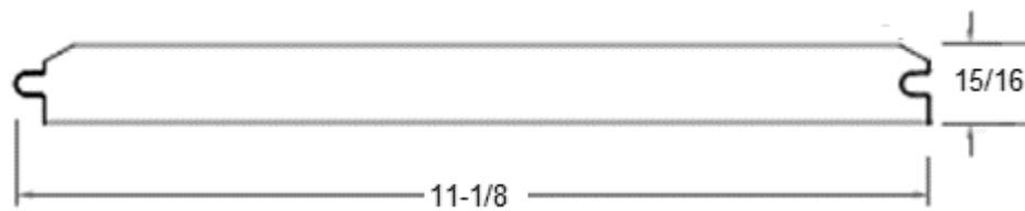
FIGURE 2 – DURATION CASTLE BLOCK SIDING
