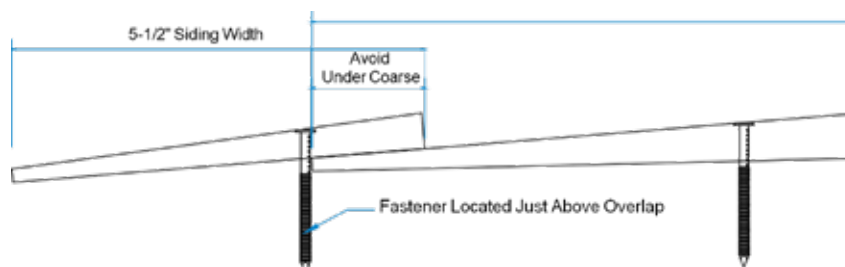
Figure 2: Face Nailing
